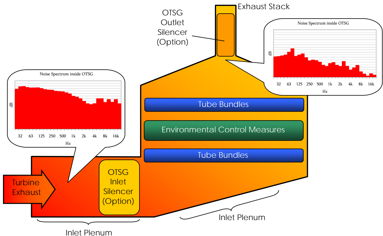
Figure 2: Once Through Steam Generator (OTSG) general Schematic. 1/3 rd Octave sound level spectra shown were obtained using a calibrated high temperature microphone assembly with an anechoic termination.
